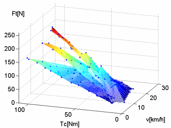
Figure 13: Traction force of the Yamaha Easy
